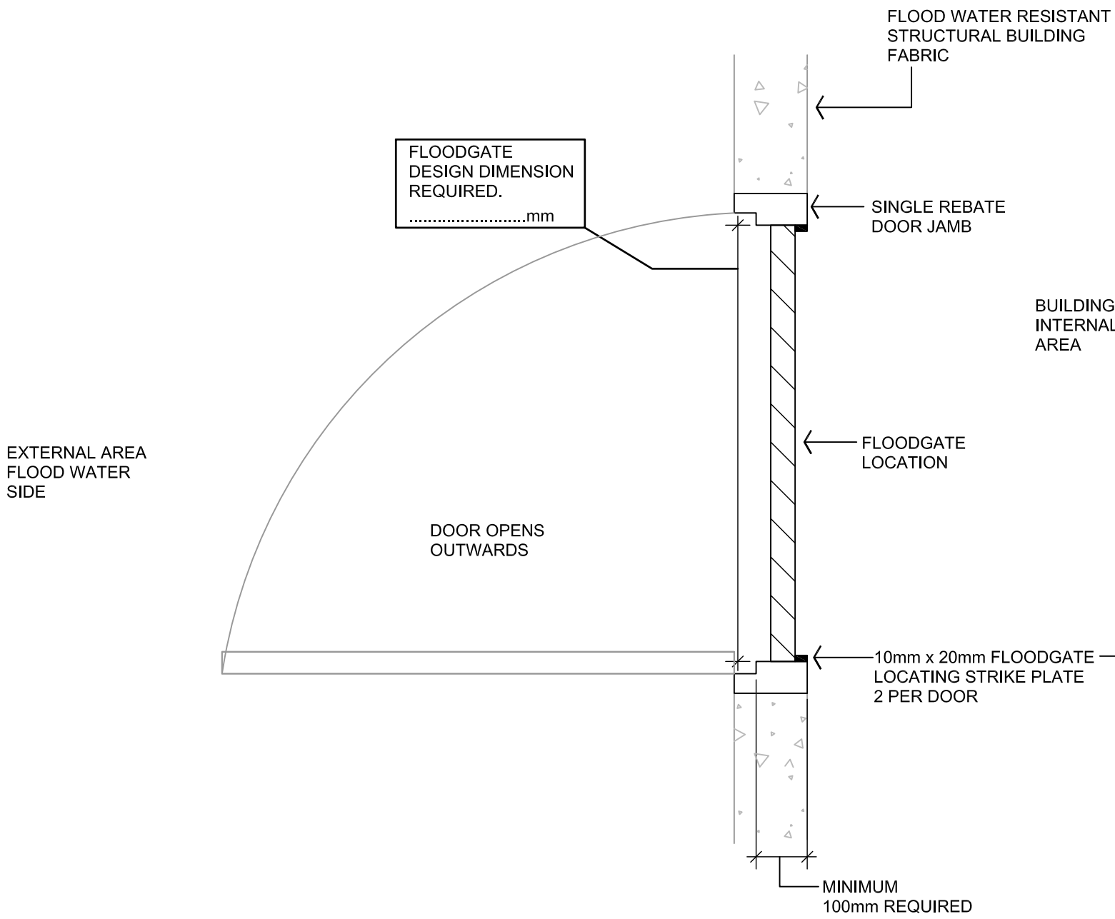
FLOODGATE DOOR TYPE OPTION 1
